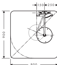
Shower installation
