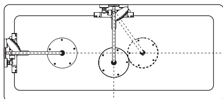
Bath tub installation
