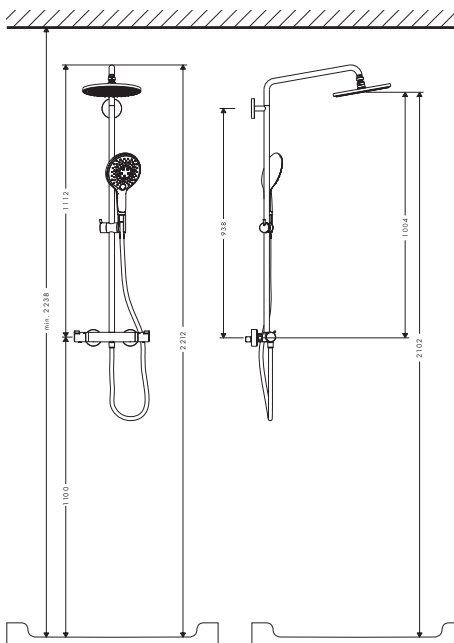
Room height B
