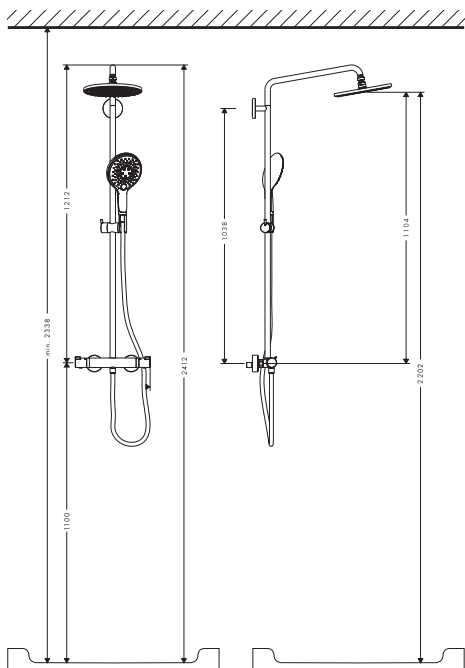
Room height A
